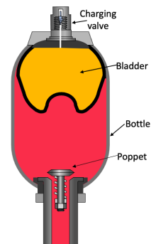
Bladder Accumulator, Fully Charged
