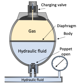
Diaphragm Accumulator Before Precharge
