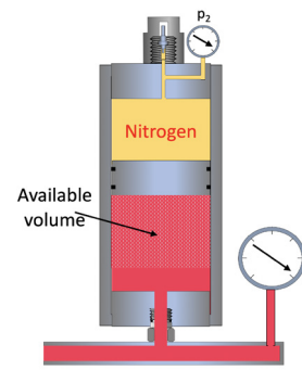
Maximum Accumulator Pressure, Maximum Stored Energy
