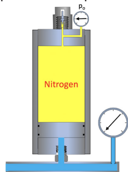
Precharge Pressure, No Stored Energy
