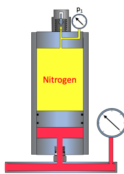
Minimum System Pressure, Minimal Stored Energy
